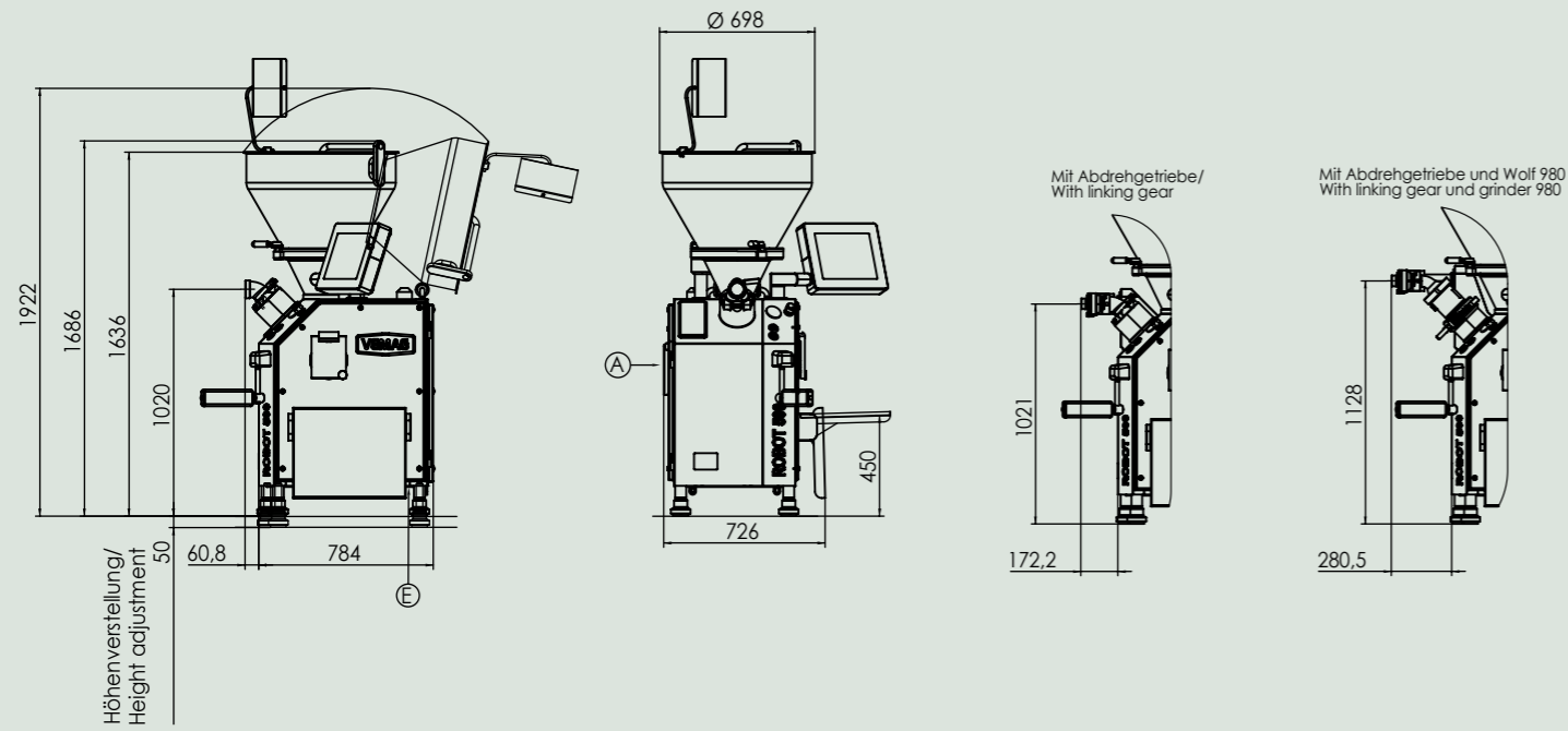
Technical drawing
